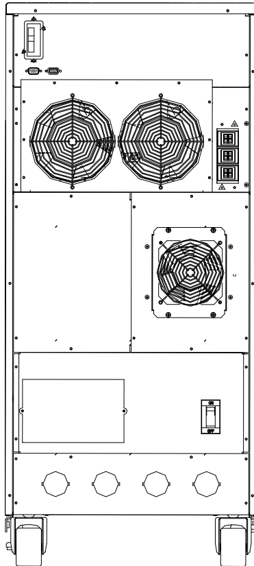
1600EP 14/18kVA UPS
